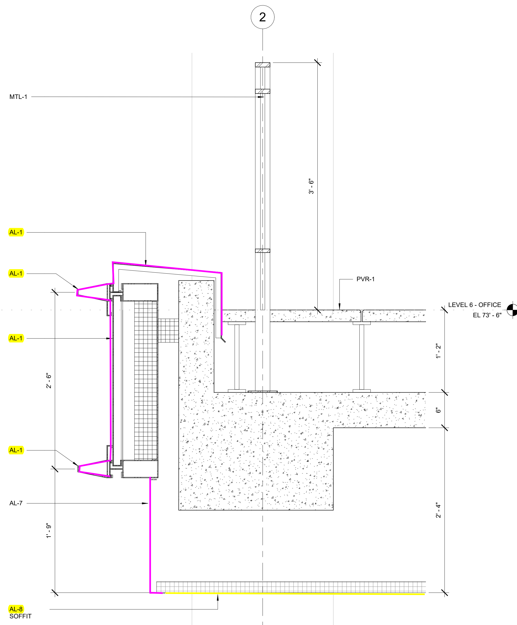
2 METAL PANEL SPANDREL DETAIL - SECTION 1 1/2" = 1'-0"
