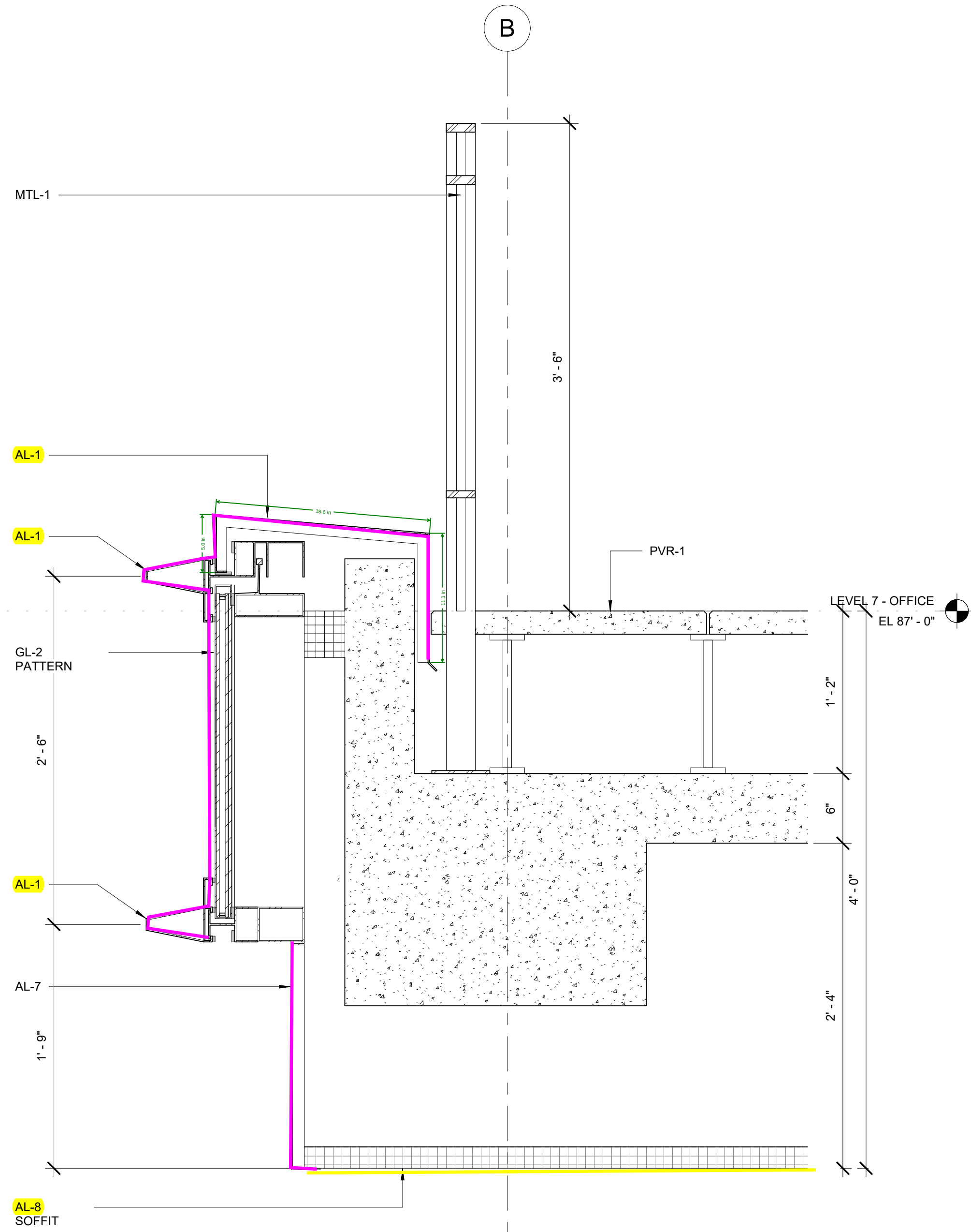
1 GLASS SPANDREL DETAIL - SECTION 1 1/2" = 1'-0"
